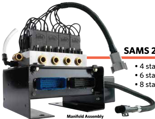
Manifold Assembly
